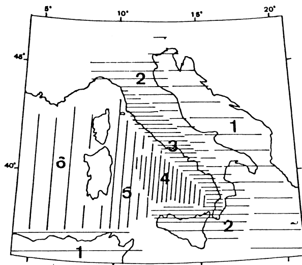
Figure 2.- Lithosphere-asthenosphere properties.
