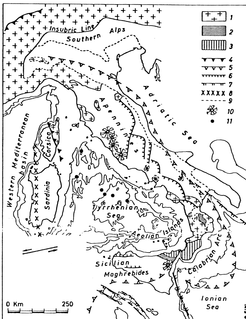
Figure 1. - Structural sketch of the circum-Tyrrhenian area. 1. Pa leogene and Neogene Europe-verging Alpine chain; 2. "Insubric" Africa-verging basement nappes; 3. Upper crystalline units of A-spromonte and Peloritani; 4. European front of the Alpine chain; 5. Neogene compression front of the Apennines and Sicilian Maghrebides. In the Ionian Sea: front of the Calabrian Ridge; 6. Neogene front of the carbonate units in the Apennines and Sicily; 7. Apulia escarpment, Malta escarpment and Pantelleria Graben; 8. Oligocene-Miocene calc-alkaline arc of western Sardinia; 9. Limits of postorogenic deposits; 10. Main uppermost Tertiary-Quaternary volcanoes on land; 11. Location of samples possibly indicating elements of the Alpine chain.
