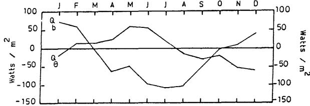
Fig.1. Annual cycle of the heat storage Q g and the advected heat flux Q b in El-Mex Bay.
