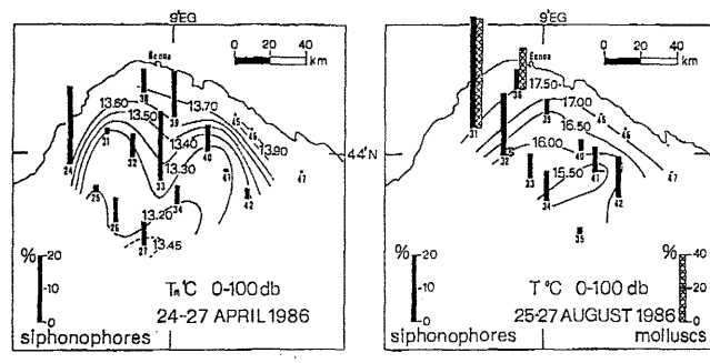
Position of sampling stations, mean isothermal for 0-100 db layer and percentage distribution of biomass (mgDW/100cm) for offshore stations.
