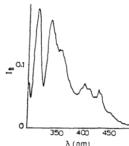
Fig. 4. Typical synchronous fluorescence spectrum (Δλ=4nm) of PAHs extract in hexane, from Saronikos gulf sediments.
