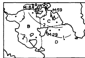
Fig. 1. Surface distribution of DDPH (µg/L) and values of PAHs in mussels (M:µg/g) from Saronikos gulf in chrysene equivalents.
