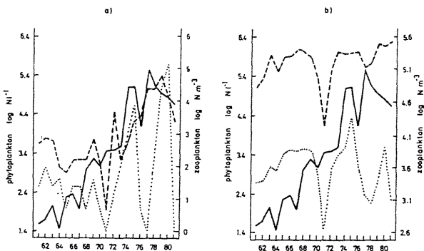
Fig. 1 Multiannual fluctuations in a) Cladocera (---) and Thaliacea (.....) b) Copepoda (---) and Appendicularia (.....) density in relation to phytoplankton fluctuations (—) (Stoncica, annual means 1961-1981).
