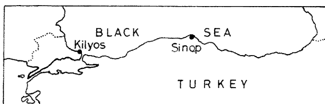
Fig. 1. The collection sites for Black Sea sediments.
