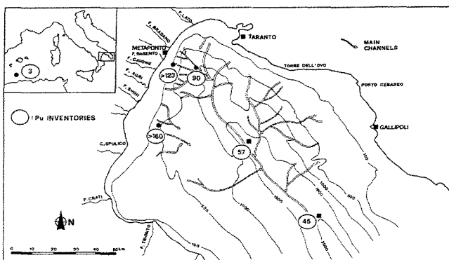
Fig. 1 - Inventories of ^{239,240}\text{Pu} ( \text{Bq/m}^2 ) in sediments of the Gulf of Taranto (main figure) and in the Algerian Basin (upper left square).
