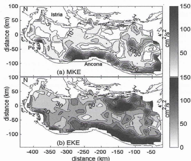
Fig. 1. Mean kinetic energy (a) and eddy kinetic energy (b) in the rotated Northern Adriatic for the period 21 September 2002 to 1 October 2003. Only bins with more than 10 observations have been taken into account.
