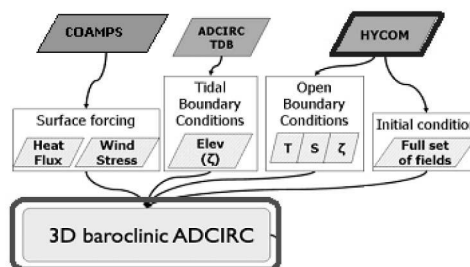
Fig. 2. The ADCIRC-HYCOM coupled model system.
