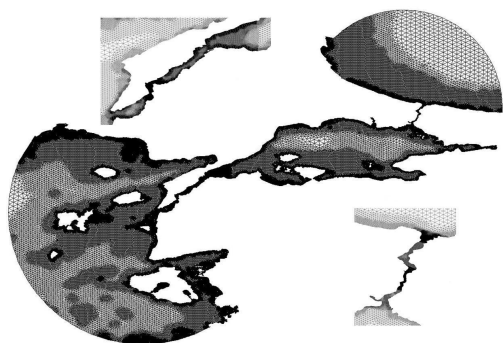
Fig. 1. ADCIRC finite element model domain for the Turkish Strait System including a zoom of the mesh refinement in the Dardanelles Strait (upper left) and Bosphorus Strait (lower right).
