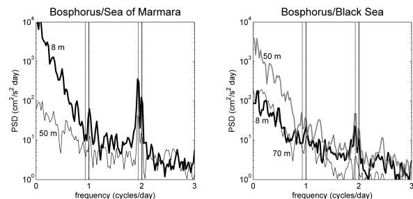
Fig. 2. As in Figure 1, but for the Bosphorus Strait.
