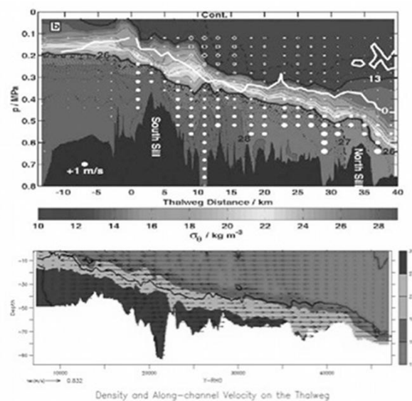
Fig. 1. Observed (top) and simulated (bottom) velocity and density distribution along the thalweg of the Bosphorus Strait.
