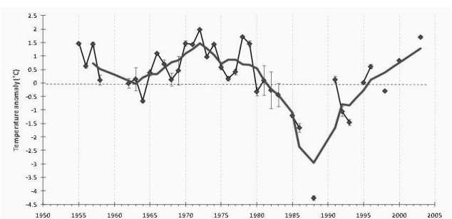
Fig. 2. Temperature anomalies aggregated over the shelf volume of 'locked' waters (as defined by \sigma_\theta=14.2 ) and averaged over summer months (May-November) shown as function of time + 5yr running mean. Error bars = 1 standard deviation.
