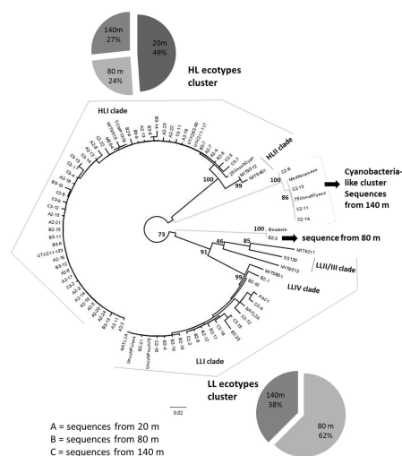
Fig. 1. ML phylogenetic tree showing the relationships of Prochlorococcus HL and LL ecotypes and clades, as well as the Cyanobacteria-like cluster. Branch support values of >75% are indicated.
