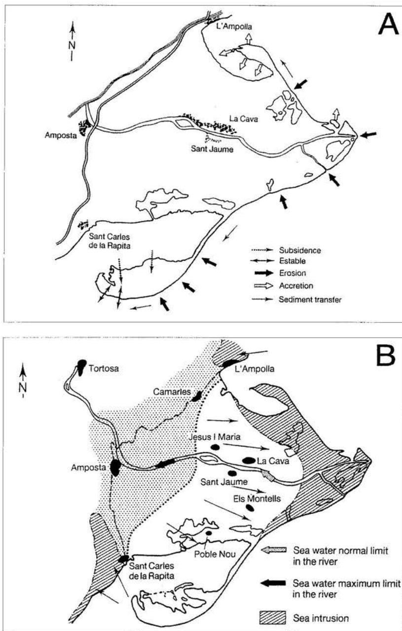
Figure 6 – Maps of the Ebro delta (after MARINO, 1992) showing (A) coastal current modified physiography and (B) sea-water intrusion in the outer quarter of this depo-center induced by subsidence. Stippled area shows highland backing delta; dotted line denotes the approximate mainland-delta boundary.
