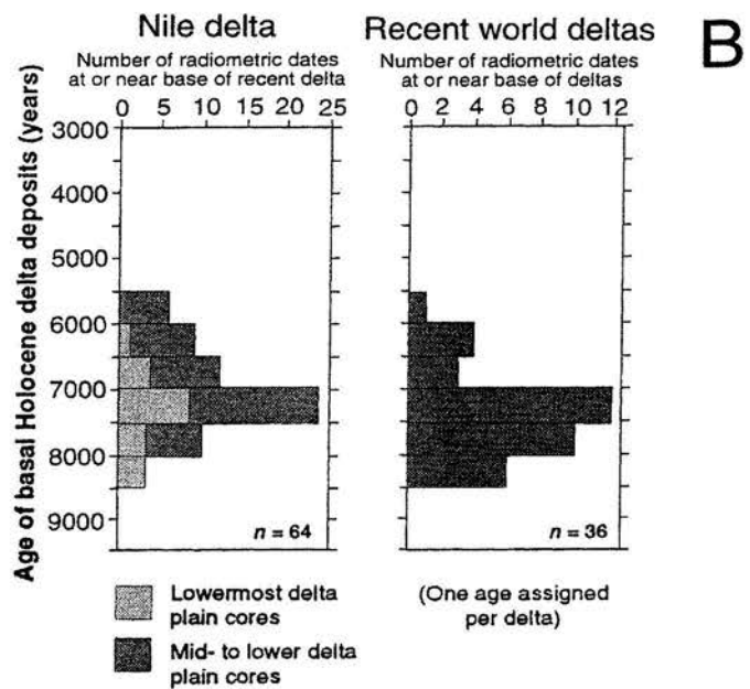
Figure 4 – A: world sea-level curve (modified from FAIRBANKS, 1989) showing initiation of rapid sea-level rise (WCT), Younger Dryas (YD), and worldwide delta initiation (DI). B: histograms showing Holocene dates at the base of sections in the Nile and other world deltas (modified from STANLEY and WARNE, 1994).
