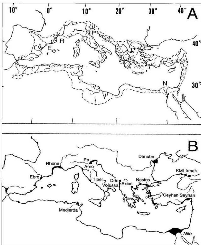
Figure 1 – A : moderate to large rivers flowing into the Mediterranean (E = Ebro, R = Rhône, P = Po, N = Nile). B : position of the largest coastal plains and major deltas cited in this study. Both modified from JEFTIC et al. (1992).
