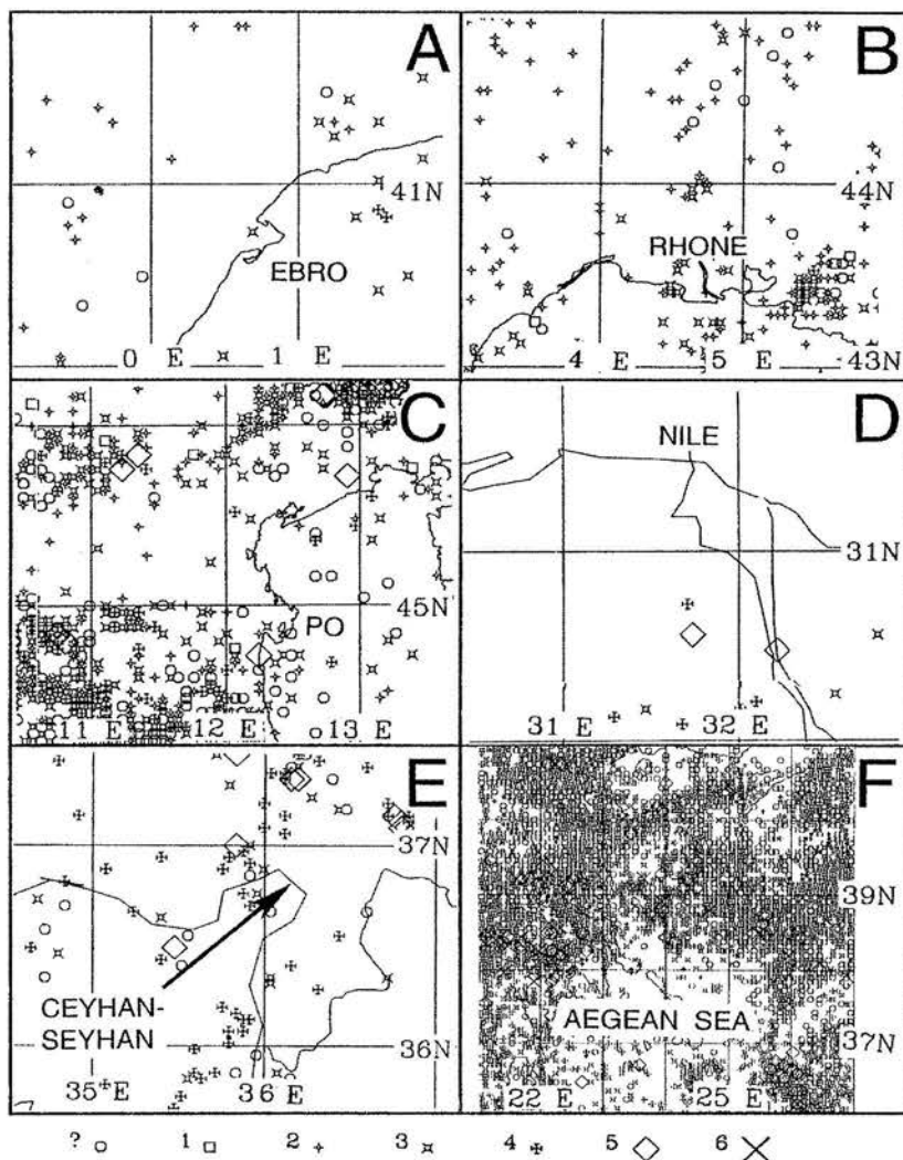
Figure 2 -- Earthquake epicenters in the vicinity of deltas discussed in this study (after REAGOR, 1996). A: Ebro (December 1968-October 1996); B: Rhône (June 1972-October 1996); C: Po (January 1950-November 1996); D: Nile (April 1974-October 1996); E: Ceyhan-Seyhan sector, with arrow pointing to Gulf of Iskenderun (March 1945-June 1996); F: Aegean Sea (March 1933-December 1996). Legend for magnitude of epicenters (Richter scale) shown at bottom.
