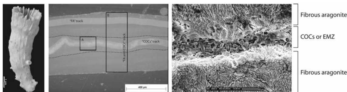
Figure 2. Left: Desmophyllum dianthus in lateral view showing the well-developed radially symmetric S1 septa. Middle and right: reflected light microscope and SEM images of a transversally sectioned S1 septum, showing rounded aggregates of aragonite crystals surrounded by bundles of fibrous aragonite. SEM image is an enlargement of the inner septal portion (A). Dashed lines represent a distinct border between deposits of centre of rapid accretion ( sensu Stolarki, 2003) and thickening deposits. The laser ablation transects along the fibrous aragonite portion and the centres of calcification were obtained using a 80µm diameter spot following the growth direction (light grey lines). Rectangle B represents the laser ablation (20x220µm slit) track crossing the FA and COCs.
