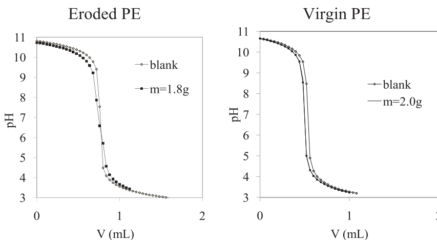
Figure 8. Potentiometric mass titrations of beached eroded PE and virgin PE pellets in NaNO 3 solution using HNO 3 . m refers to the mass of pellets titrated.
