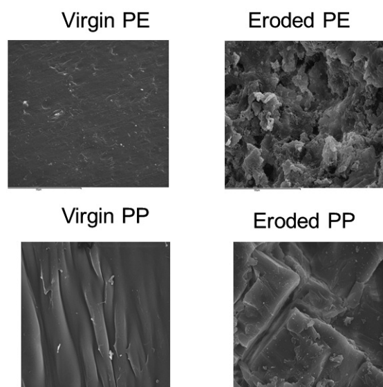
Figure 5. The surface topography of virgin plastic pellets from SEM for virgin and beached, PE and PP pellets enlarged 1000 times (Note the gray scale bar at the bottom of the image; scale bar 60 μm).
